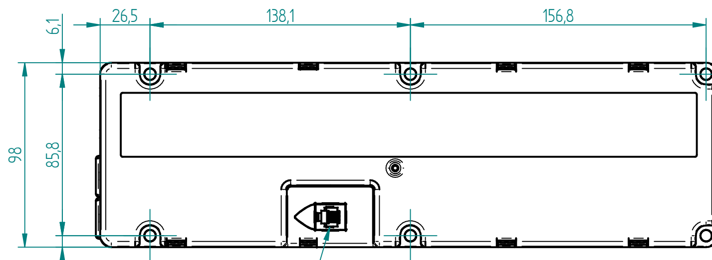
Handtaster Hand switch
