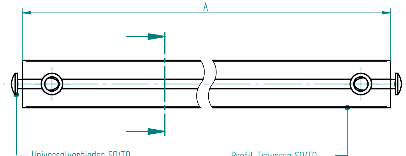
Universalverbinder SQ/TQ Universal fastener SQ/TQ 142.00210 (2x)
